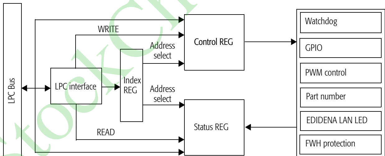
Figure 9. EPLD block diagram
