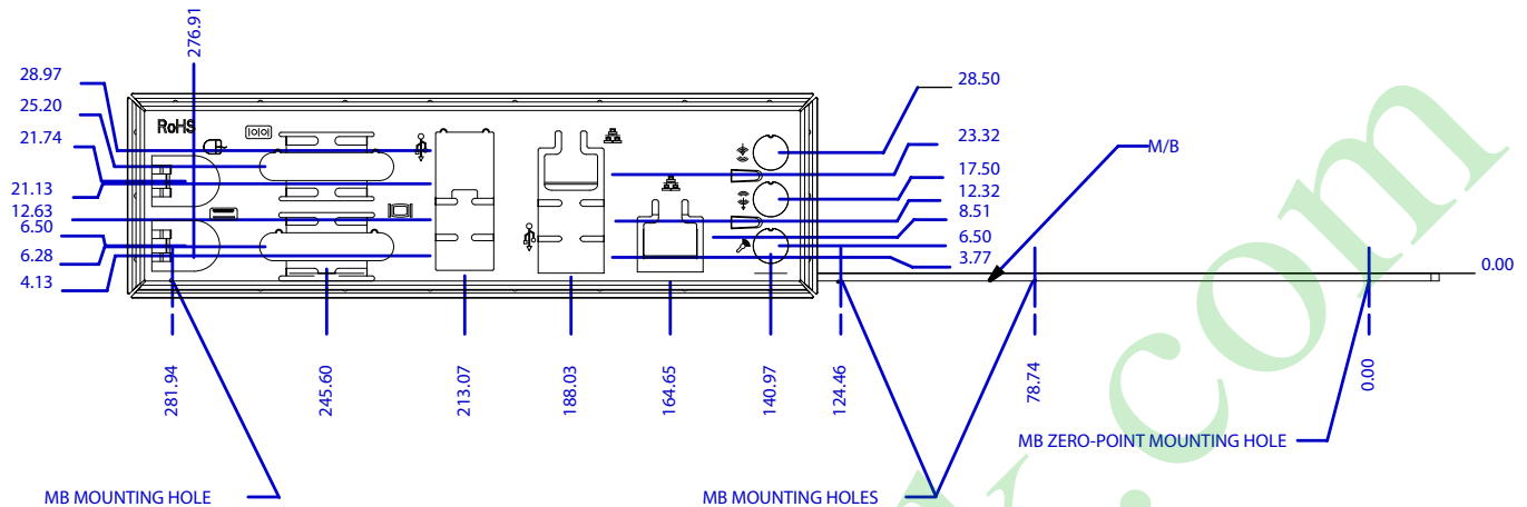
Figure 6. I/O shield for the JD35Q and QZ35Q motherboards
